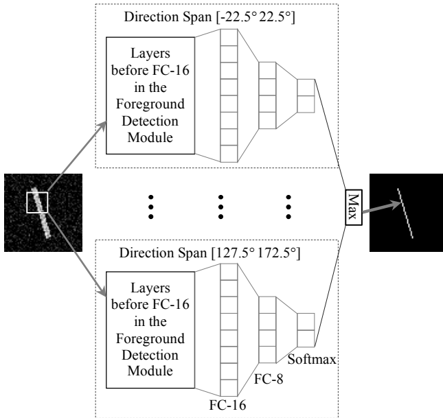
Figure 7. Centerline extraction neural network module.
