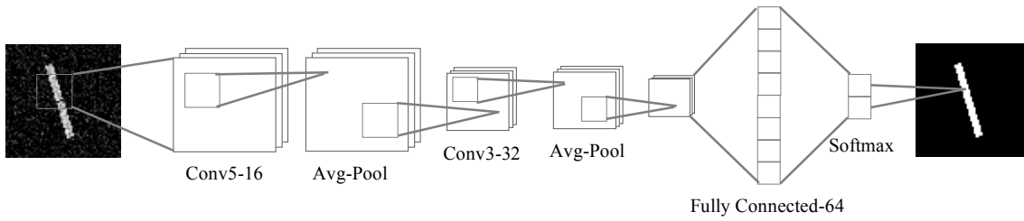
Figure 4. A trial CNN architecture for foreground detection.
