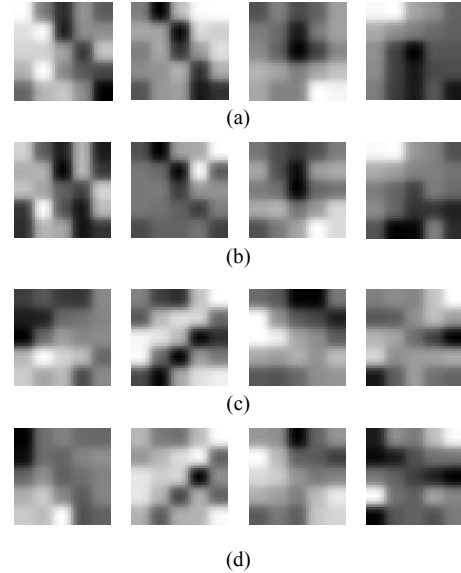
Figure 8. (a) & (c) Weights of a few neurons in the foreground detection CNN responsible for 30^\circ and 150^\circ , respectively. (b) & (d) Weights of the neurons in the centerline extraction CNN corresponding to the neurons in (a) & (c).
