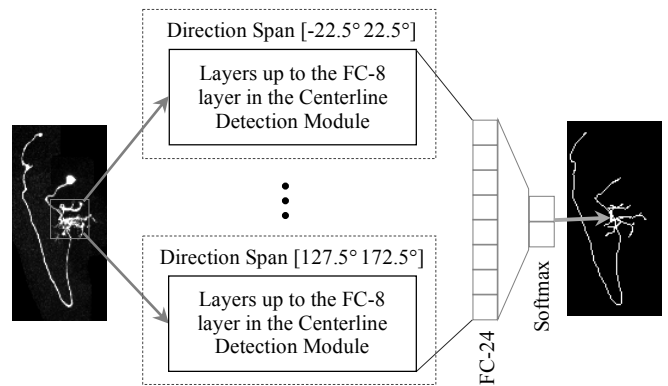
Figure 9. Deep-Transfer-Learning neural network architecture.
