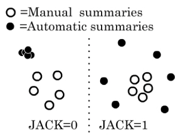
Figure 4: JACK values
