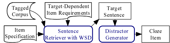
Figure 2: Main components of our item generator
