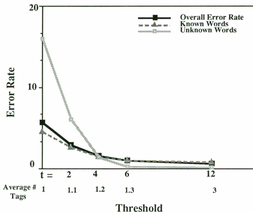
Figure 4: Comparison of thresholds for K- Best
