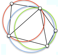
Figure 1. A Delaunay mesh. Note that the circumcircle for each of the triangles does not contain other points in the mesh.
