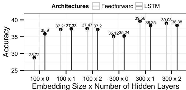
Figure 4: Comparison between feedforward and sequential LSTM when using summation pooling function.
