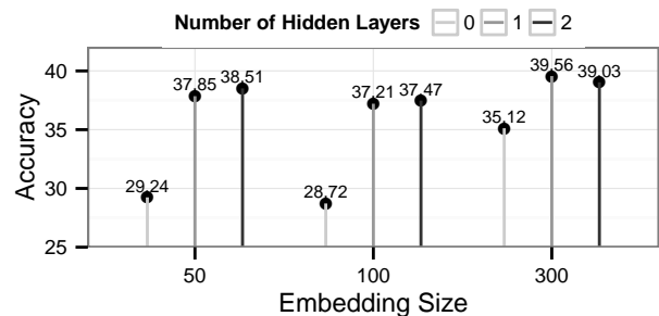
Figure 3: Inter-argument interaction can be modeled effectively with hidden layers. The results are shown for the feedforward models with summation pooling, but this effect can be observed robustly in all architectures we consider.
